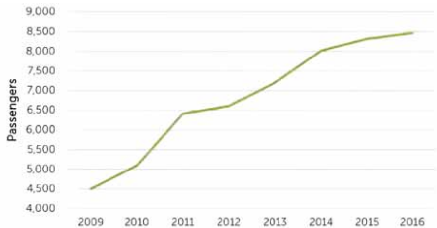
Figure 2.37 Amtrak Ridership
