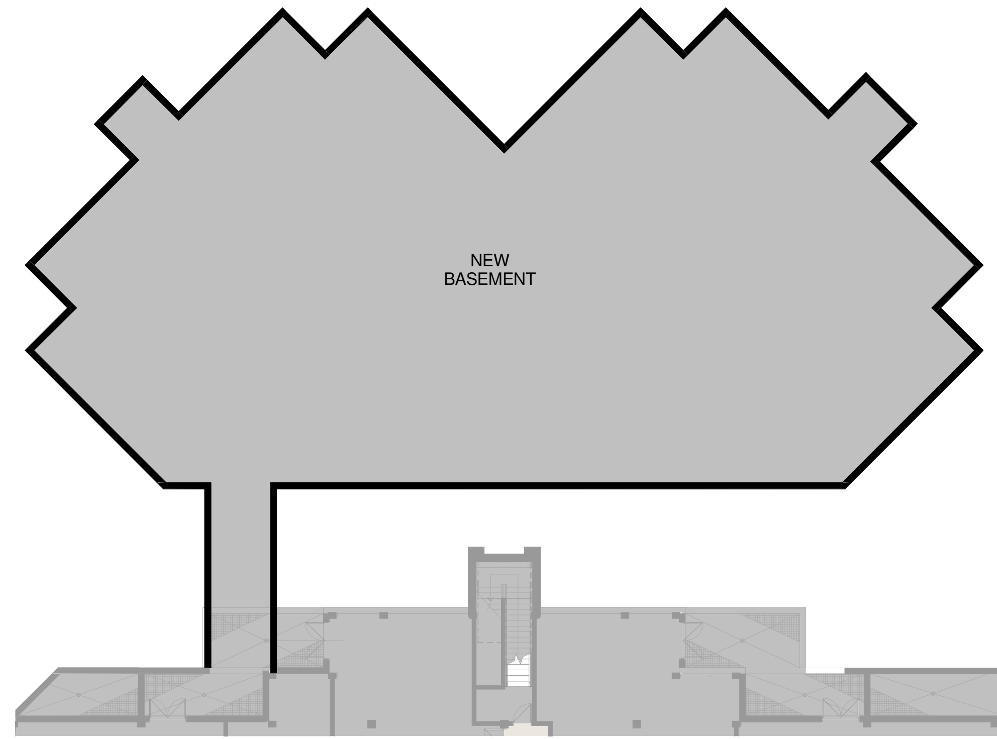
BASEMENT FLOOR PLAN 1/16" = 1'-0"
